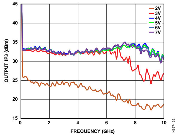
Figure 32. Output IP3 vs. Frequency for Various Supply Voltages, P_{OUT}/Tone = 5 \text{ dBm}
