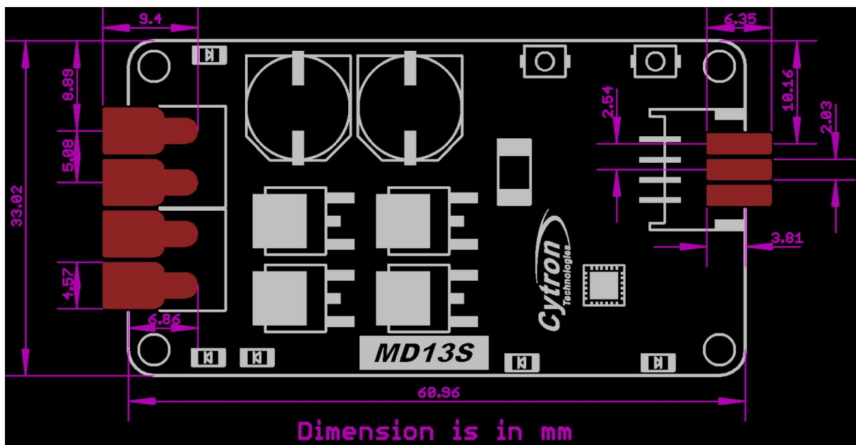
Footprint Dimension
