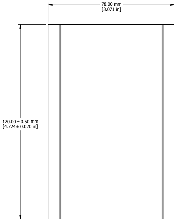
EXTRUSION
