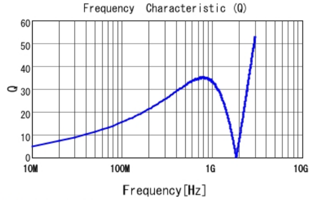
■ LQG18HN33NJ00 Q
