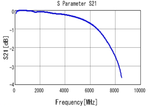
■ GRM1885C2A820JA01 S21 DCOV, 25degC
