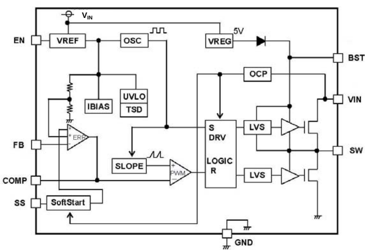
Figure 3. Block Diagram
