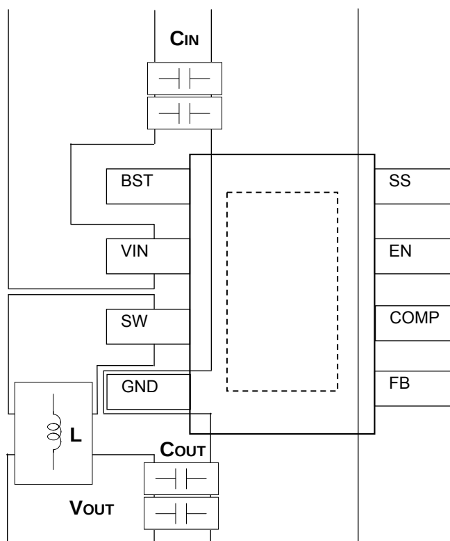
Figure 27. An example of PCB Layout Pattern
