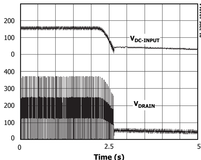
Figure 13. Slow Power-down Timing with Optional External (2 M \Omega ) UV Resistor Connected to EN/UV Pin.
