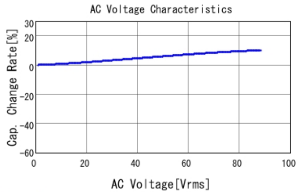
GRM188R72E152KW07 C-AC Voltage capchange, DCOV, 25
