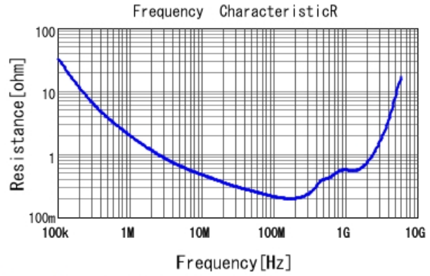
GRM188R72E152KW07 R DCOV, 25degC
