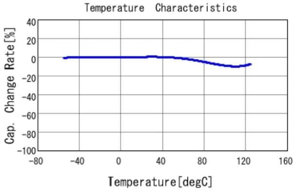
GRM188R72E152KW07 C-Temp. capchange, DCOV, AC1Vrms
