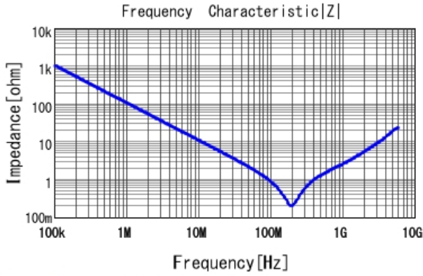
GRM188R72E152KW07 |Z| DCOV, 25degC
