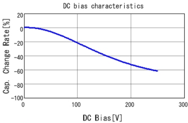
GRM188R72E152KW07 C-DC bias capchange, 25.0degC, A
