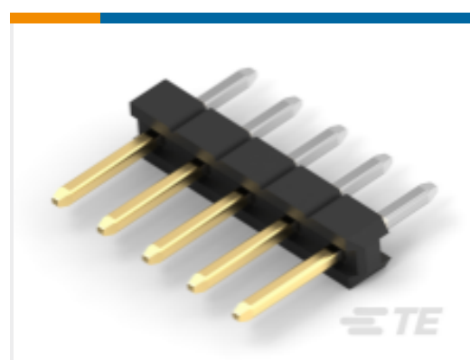
TE Part #2355172-5 5P,2MM,BRK HDR,SRVT,2.8,0.1AU,BOX
