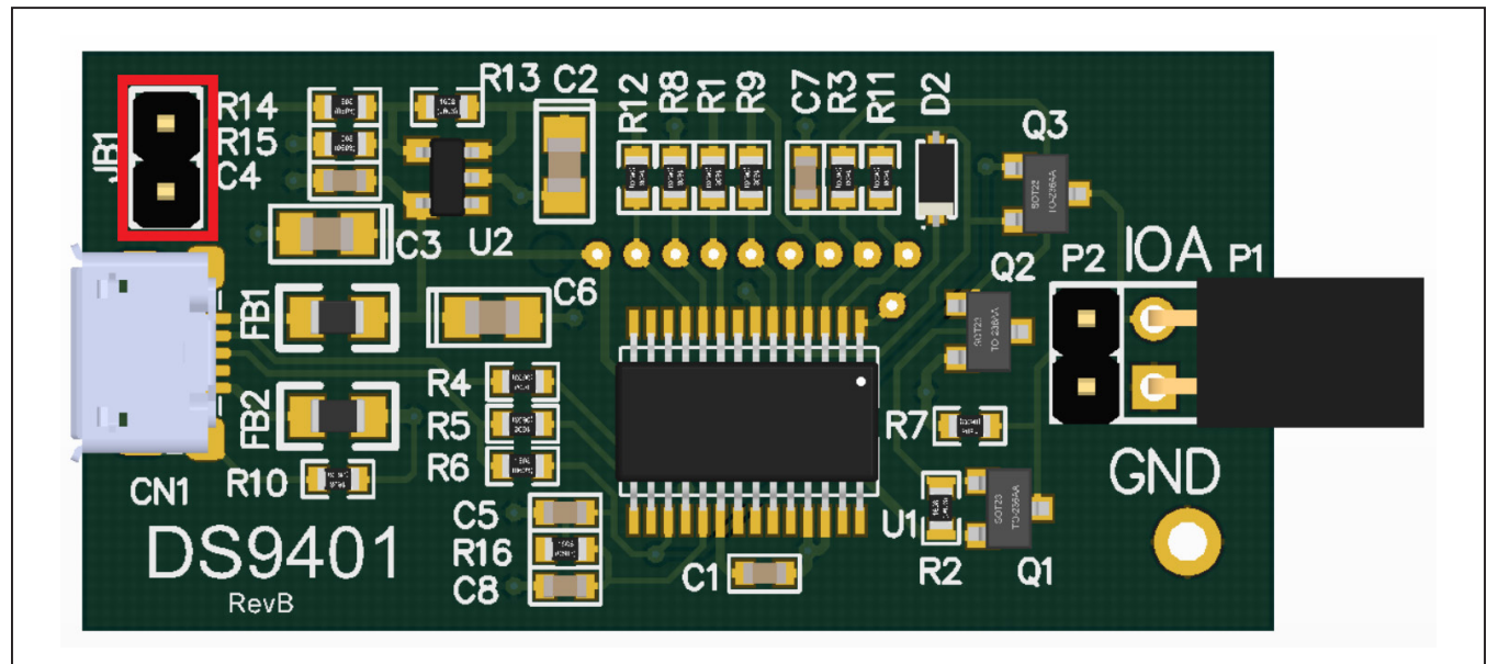
Figure 2. DS9401 Board
