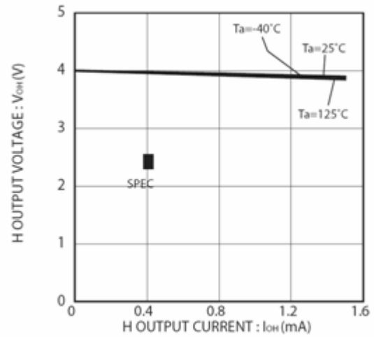
Figure 6. H output voltage V_{OH} - I_{OH} ( V_{CC}=4.0\text{V} )
