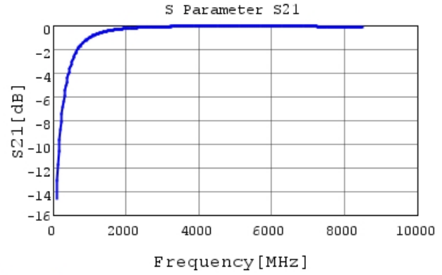
GRM0335C1E3R0BA01 S21 DCOV, 25degC
