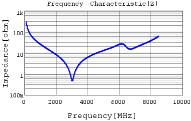
GRM1885C1H5R6DA01 |Z| DCOV, 25degC
