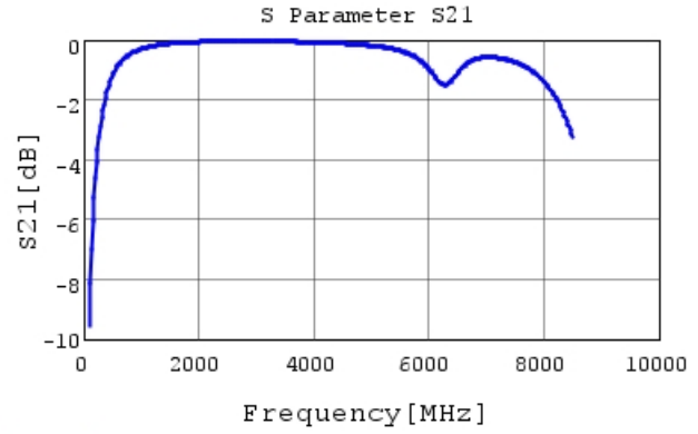
GRM1885C1H5R6DA01 S21 DCOV, 25degC
