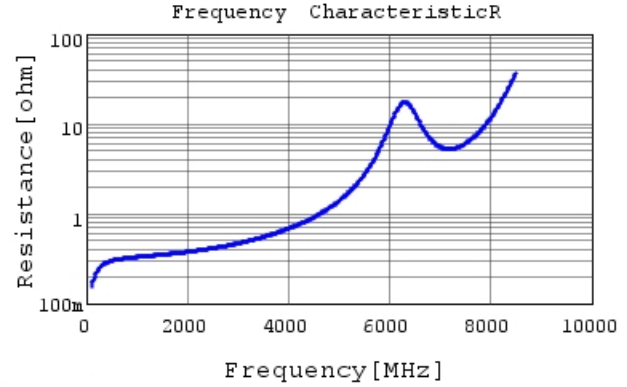
GRM1885C1H5R6DA01 R DCOV, 25degC
