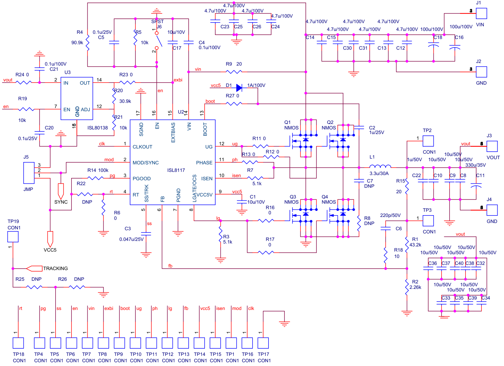
FIGURE 20. ISL8117EVAL2Z SCHEMATIC
