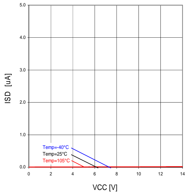
Figure 26. V_{CC}-I_{SD} ( V_{EN}=0V )
