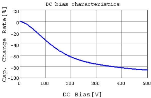
GRM32DR72H104KW10 C-DC bias capchange, 25.0c
