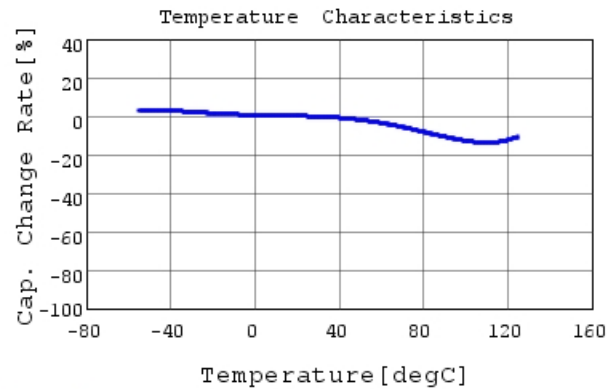
GRM32DR72H104KW10 C-Temp. capchange, DCOV, 1
