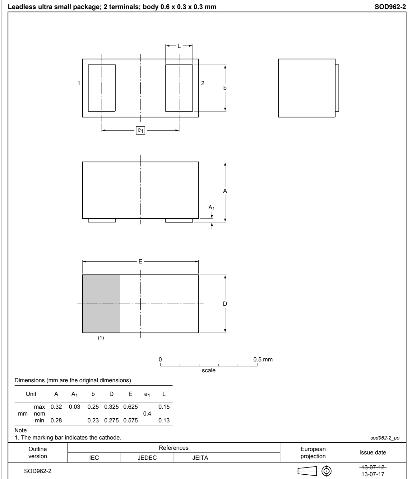
Fig. 13. Package outline DSN0603-2 (SOD962-2)
