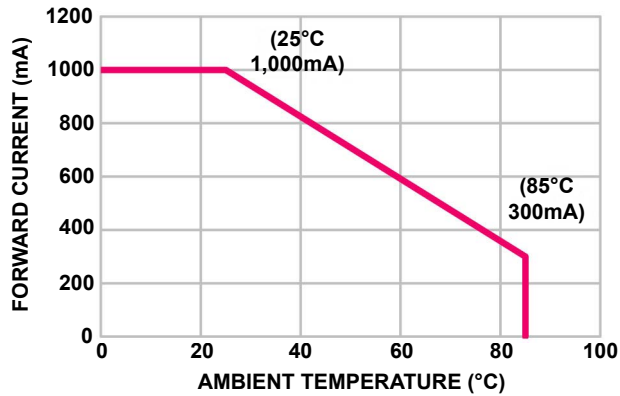
TEMPERATURE DERATING CURVE (Tj < 130°C, ~ 32°C/W) (Ambient Temperature vs. Allowable Forward Current)
