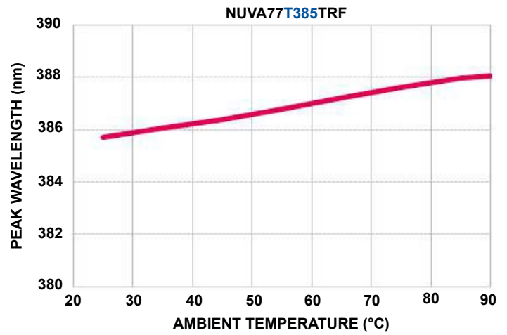
AMBIENT TEMPERATURE VS. PEAK WAVELENGTH @ 500mA If
