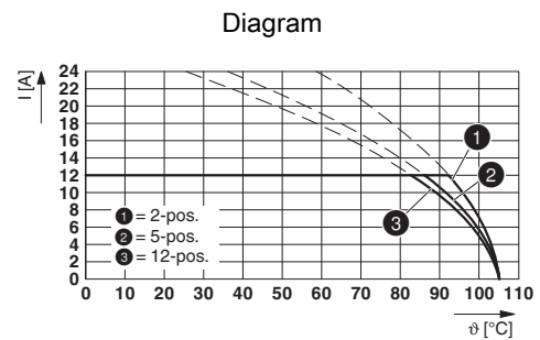
Type: GFKC 2,5/...-ST-7,62 with GMSTB 2,5/...-G-7,62
