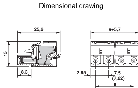
Type: GFKC 2,5/...-ST-7,62 with GMSTB 2,5/...-G-7,62
