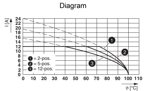
Type: MVSTB(R/W) 2,5/...-STF-5,08 with CC 2,5/...-GF-5,08-LR P...THR
