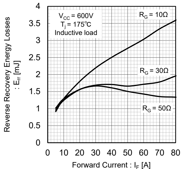
Fig.20 Typical Diode Reverse Recovery Energy Losses vs. Forward Current
