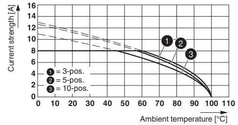
Type: MCVR 1,5/...-ST-3,81 with MCO 1,5/...-GR-3,81
