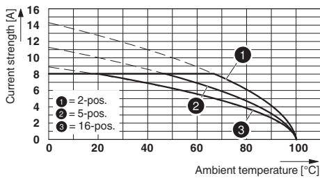
Type: MCVR 1,5/...-ST-3,81 with MCD 1,5/...-G-3,81
