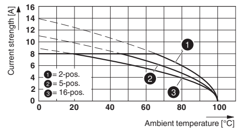
Type: MCVR 1,5/...-ST-3,81 with MCDV 1,5/...-G-3,81
