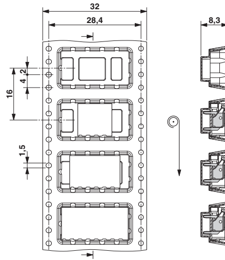
Dimensional drawing
