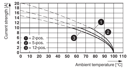
Type: FKCV(R/W) 2,5/...-ST-5,08 with MDSTBV 2,5/...-G-5,08
