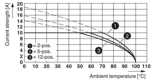
Type: FKCT 2,5/...-ST-5,08 with MDSTBV 2,5/...-G-5,08
