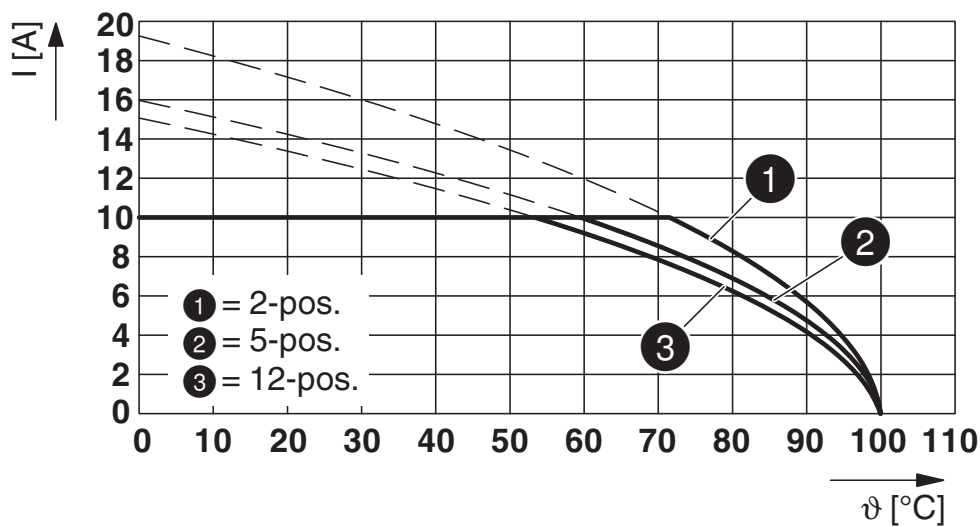
Type: FKCN 2,5/...-ST-5,08 with MDSTBV 2,5/...-G-5,08
