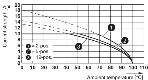
Type: MSTBT 2,5/...-ST-5,08 with MDSTBV 2,5/...-G-5,08
