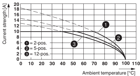
Type: MSTBP 2,5/...-ST-5,08 with MDSTBV 2,5/...-G-5,08
