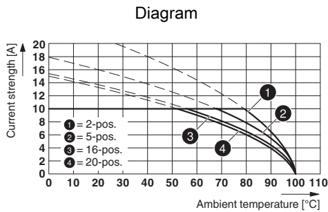
Type: MSTB 2,5/...-ST-5,08 with MDSTB 2,5/...-G1-5,08
