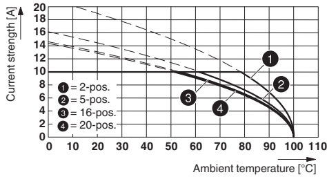
Type: MSTBP 2,5/...-ST-5,08 with MDSTB 2,5/...-G1-5,08
