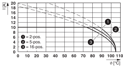
Type: FKCVR 2,5/...-ST-5,08 with MDSTB 2,5/...-G1-5,08
