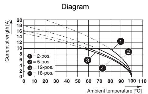
Type: MSTBT 2,5/...-ST-5,08 with MDSTB 2,5/...-G1-5,08
