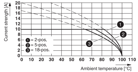
Type: FKCN 2,5/...-ST-5,08 with MDSTB 2,5/...-G1-5,08
