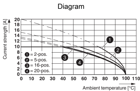
Type: SMSTB 2,5/...-ST-5,08 with MDSTB 2,5/...-G1-5,08
