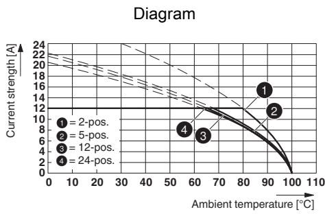
Type: MSTB 2,5/...-ST-5,08 with MSTB 2,5/...-G-5,08
