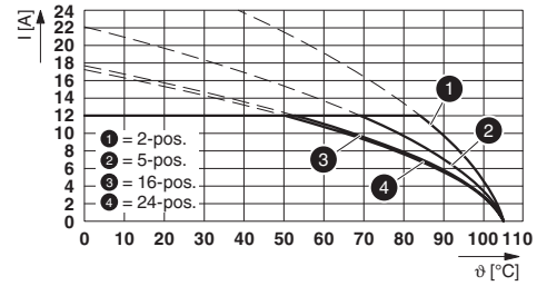
Type: ICV 2,5/...-G-5,08 with MSTB 2,5/...-G-5,08
