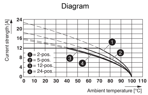
Type: MSTBU 2,5/...-STD-5,08 with MSTB 2,5/...-G-5,08
