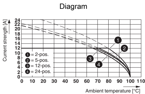
Type: MSTBP 2,5/...-ST-5,08 with MSTB 2,5/...-G-5,08
