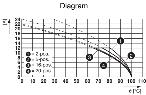
Type: FKCT 2,5/...-ST-5,08 with MSTB 2,5/...-G-5,08
