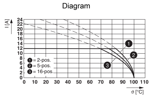
Type: FKCV(W/R) 2,5/...-ST-5,08 with MSTB 2,5/...-G-5,08
