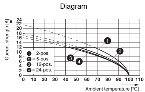
Type: SMSTB 2,5/...-ST-5,08 with MSTB 2,5/...-G-5,08
