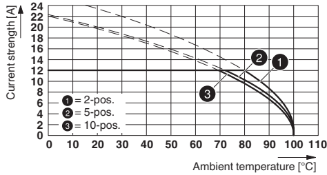
Type: TMSTBP 2,5/...-ST-5,08 with MSTB 2,5/...-G-5,08
