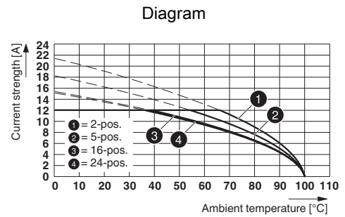
Type: MSTBP 2,5/...-ST-5,08 with MSTBW 2,5/...-G-5,08
