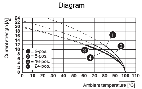
Type: MSTBP 2,5/...-ST-5,08 with MSTBA 2,5/...-G-5,08-5,08
