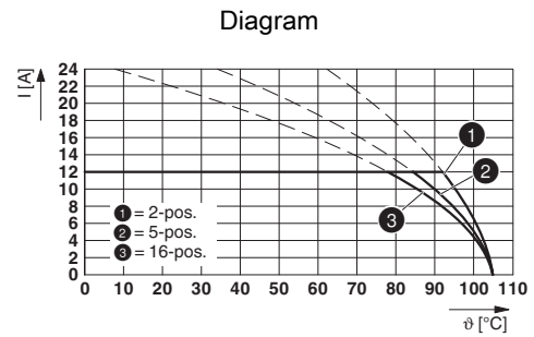
Type: FKCVW 2,5/...-ST-5,08 with MSTBA 2,5/...-G-5,08
