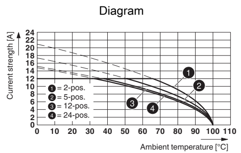
Type: MVSTBR 2,5/...-ST-5,08 with MSTBA 2,5/...-G-5,08
