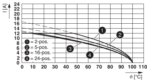
Type: SMSTB 2,5/...-ST-5,08 with MSTBVA 2,5/...-G-5,08
