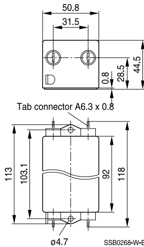
B84114D0000B110 (10 A)
