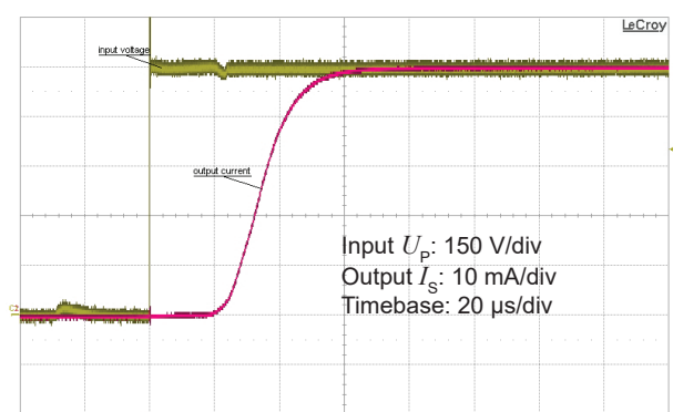
Figure 6: Typical step response (0 to 750 V)
