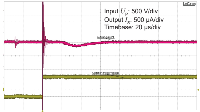
Figure 14: Detail of typical common mode perturbation (750 V step with 6 kV/μs, R_M = 100 \Omega )
