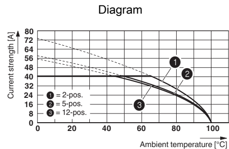
Derating curve for: PC 5/...-ST1-7,62 with PC 5/...-G-7,62 Conductor cross section: 10 mm 2
