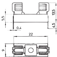
199015 approvals UL(rec), VDE
