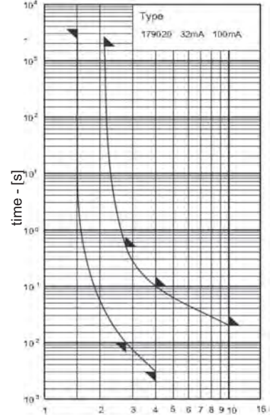
Time-Current Characteristics
