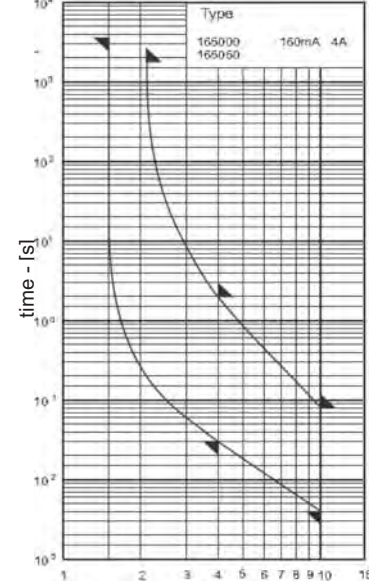
Time-Current Characteristics
