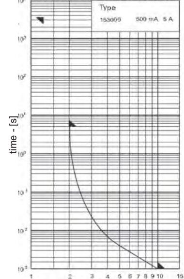
Time-Current Characteristics
