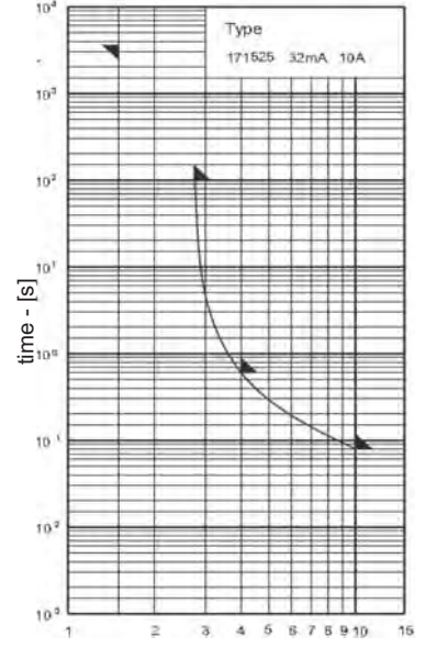
Time-Current Characteristics
