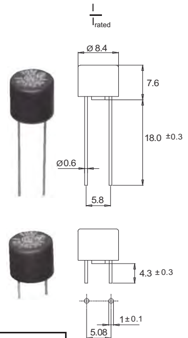
Dimensions [mm]
