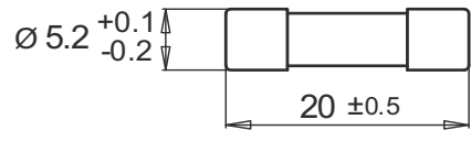
Dimensions [mm]
