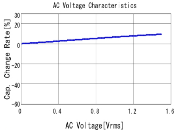
■ KCM55WR7YA476MH01 C-AC Voltage capchange, DCOV, 25.0d
