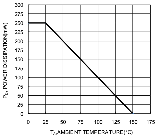
T A , AMBIENT TEMPERATURE (°C) Figure 1. Power Derating Curve
