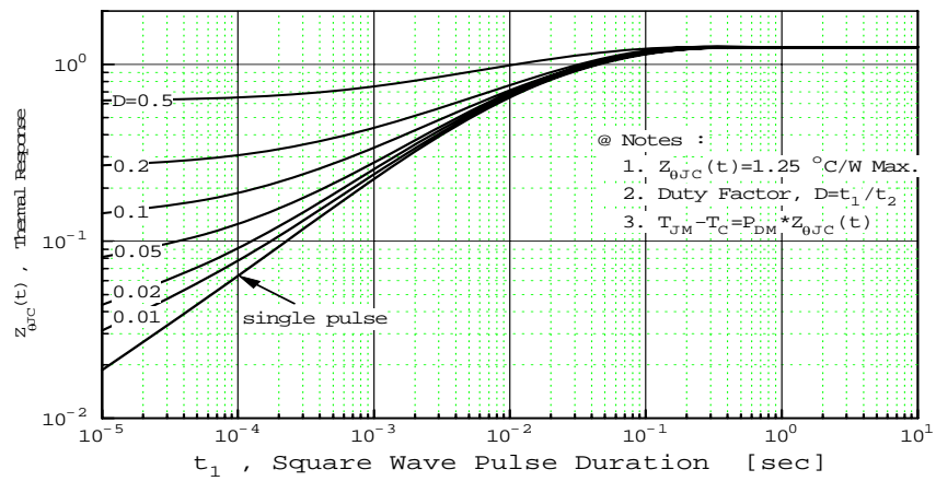
Figure 11. Thermal Response
