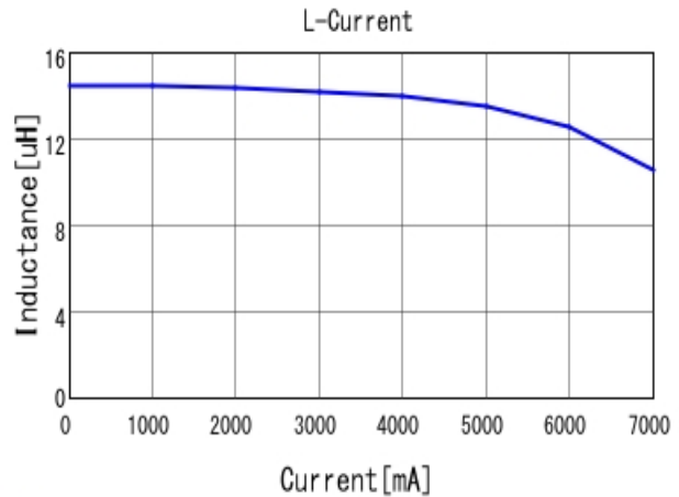
■ 1274AS-H-150M L-Current 20degC
