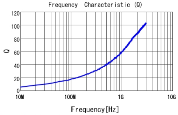
LQG18HN2N2S00 Q
