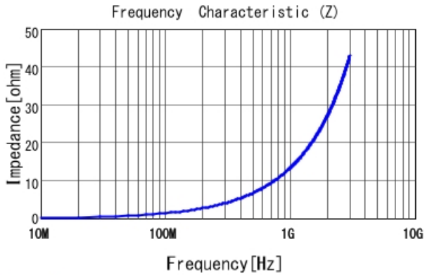
LQG18HN2N2S00 |Z|
