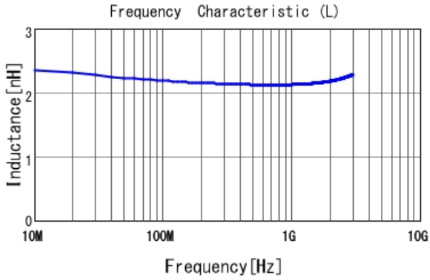
LQG18HN2N2S00 L
