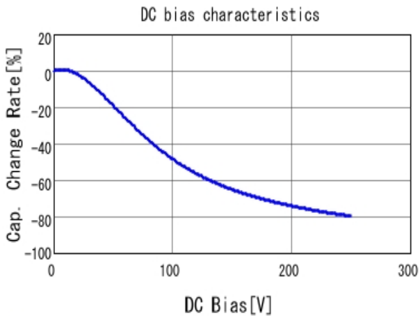
■ GRM31CR72E104KW03 C-DC bias capchange, 25.0degC, AC1V
