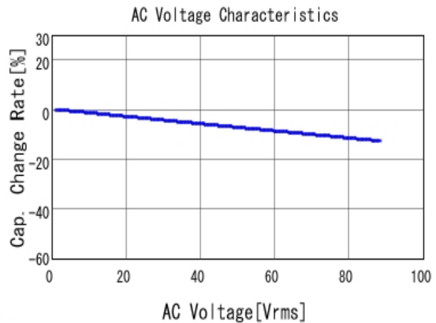
■ GRM31CR72E104KW03 C-AC Voltage capchange, DCOV, 25.0d
