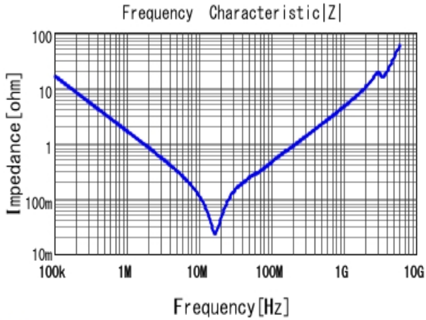
■ GRM31CR72E104KW03 |Z| DCOV, 25degC
