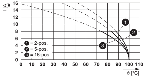
Type: MC 1,5/...-ST-3,81 with SMC 1,5/...-G-3,81
