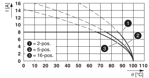
Type: MC 1,5/...-ST-3,81 with MCDV 1,5/...-G-3,81
