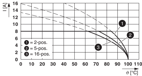
Type: MC 1,5/...-ST-3,81 with MCD 1,5/...-G-3,81
