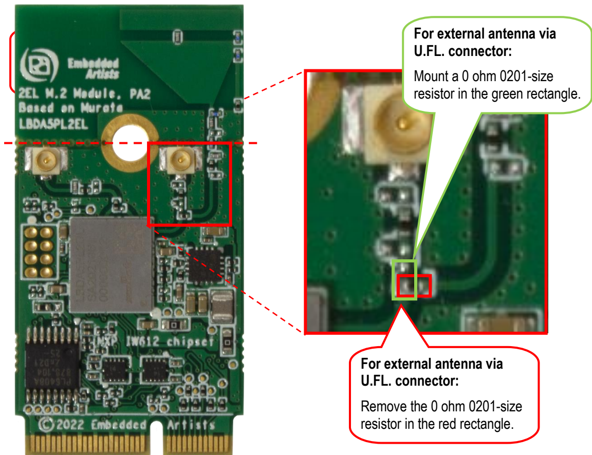
Figure 9 – Rework to Connect U.FL. Connector
