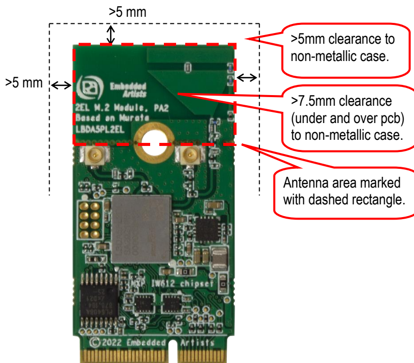
Figure 8 – M.2 Module Clearance Area
