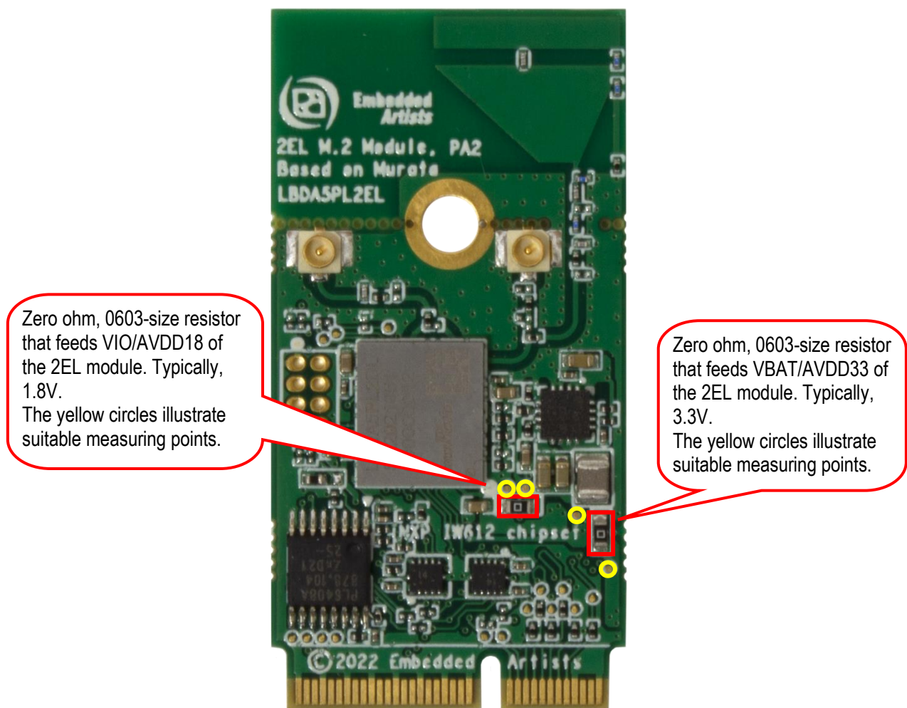
Figure 7 – Current Measurement
