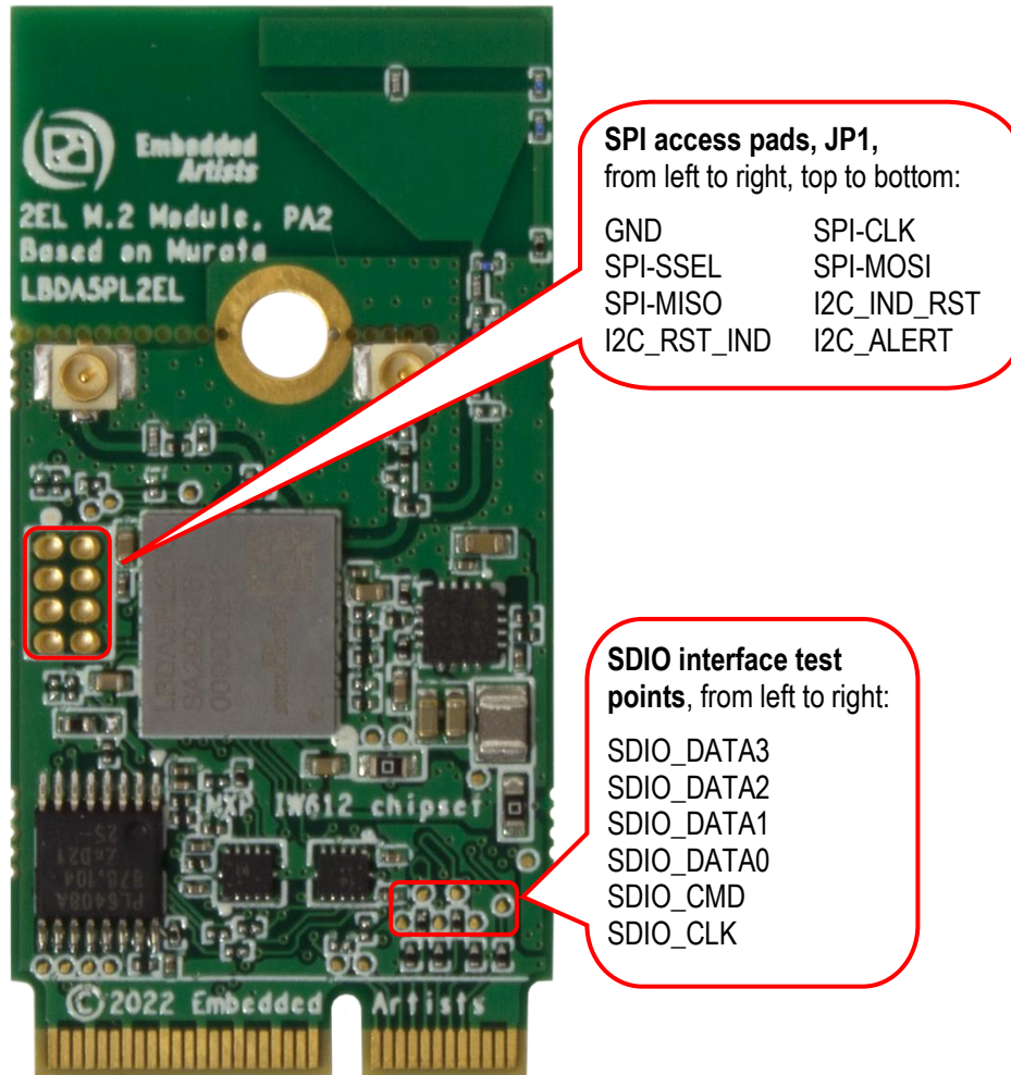
Figure 6 – 2EL M.2 Module Test Points
