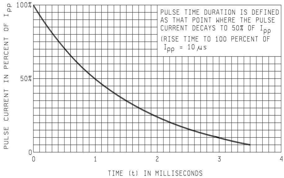
FIGURE 8. Current impulse waveform.
