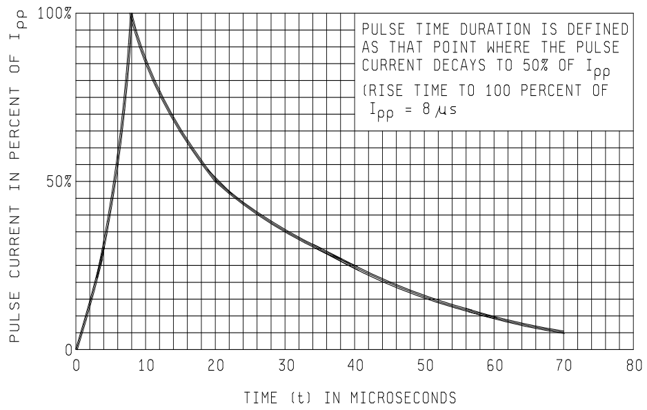
FIGURE 9. Current impulse waveform.
