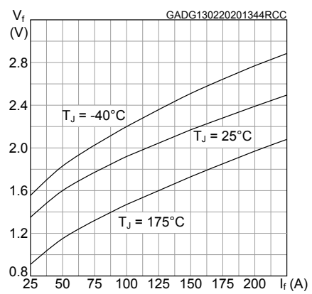
Figure 10. Diode V_F vs forward current
