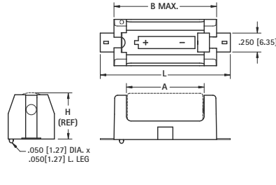
Surface Mount (SMT)
