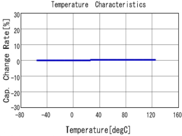
■ GRM21A5C2E270JW01 C-Temp. capchange, DCOV, AC1Vrms
