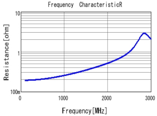
■ GRM21A5C2E270JW01 R DC0V, 25degC
