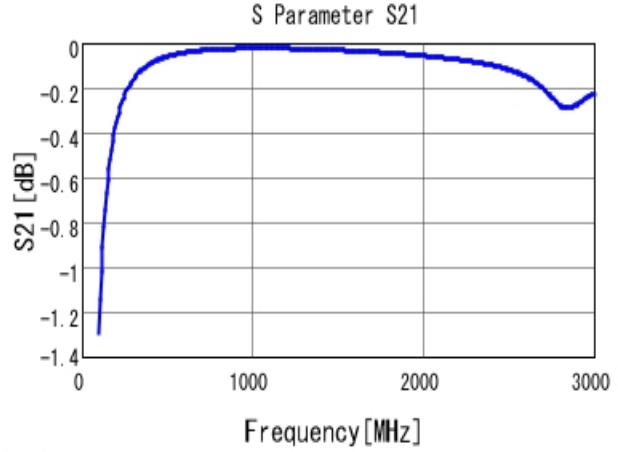
■ GRM21A5C2E270JW01 S21 DCOV, 25degC
