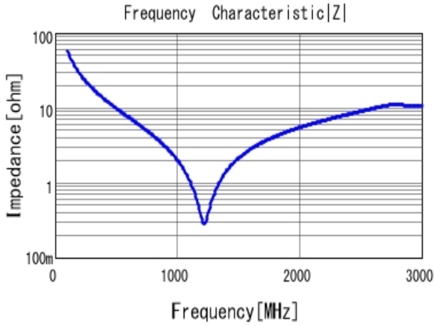
■ GRM21A5C2E270JW01 |Z| DC0V, 25degC
