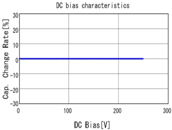
■ GRM21A5C2E270JW01 C-DC bias capchange, 25.0degC, AC1V
