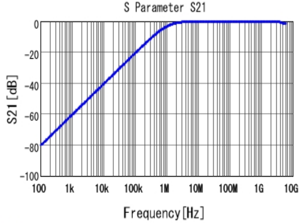
■ GRM188R72A152KA01 S21 DCOV, 25degC
