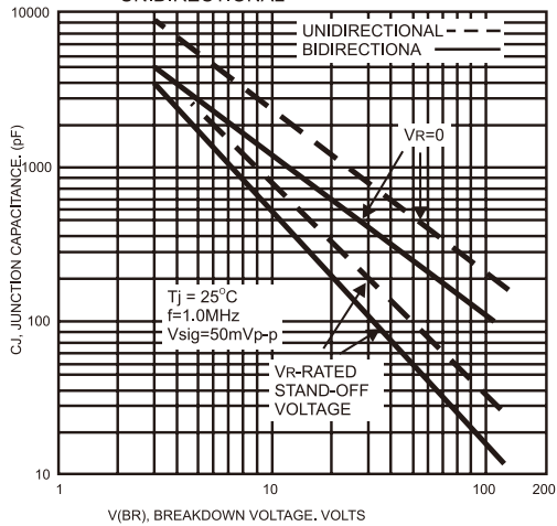
FIG.5- TYPICAL JUNCTION CAPACITANCE UNIDIRECTIONAL
