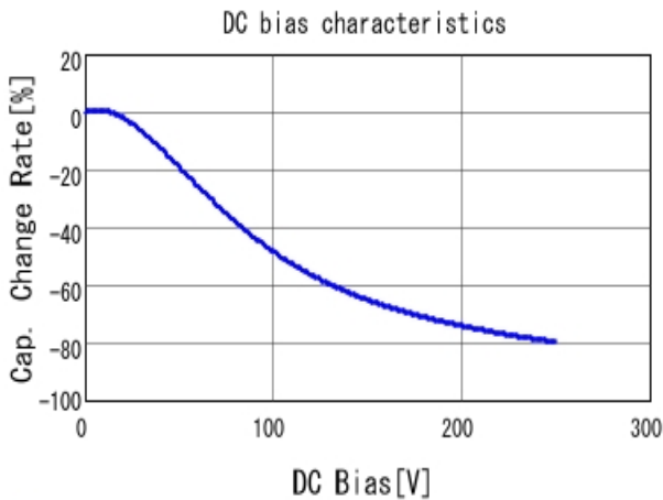
■ RDER72E104K2M1H03A C-DC bias capchange, 25.0degC, AC1
