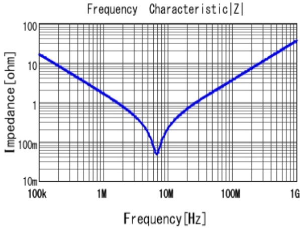
■ RDER72E104K2M1H03A |Z| DC0V, 25degC
