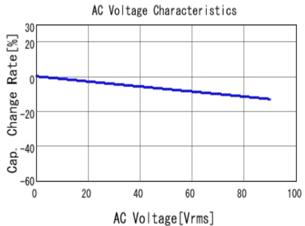
■ RDER72E104K2M1H03A C-AC Voltage capchange, DC0V, 25.0
