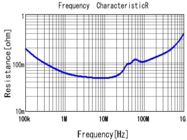
■ RDER72E104K2M1H03A R DC0V, 25degC
