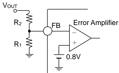
Figure 62. Feedback Resistors
